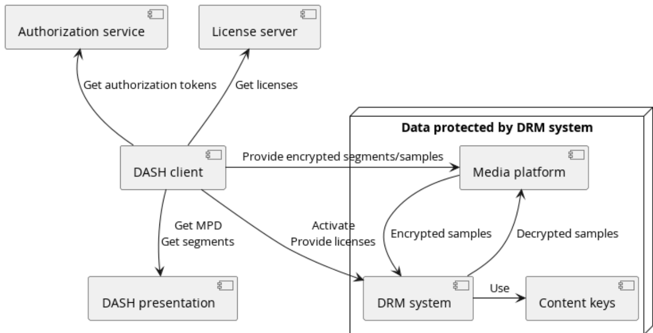
Figure 1 A DRM system cooperates with the device's media platform to enable playback of encrypted content while protecting the decrypted samples and content keys against potential attacks. The DASH-IF implementation guidelines focus on the signaling in the DASH presentation and the interactions of the DASH client with other components.
